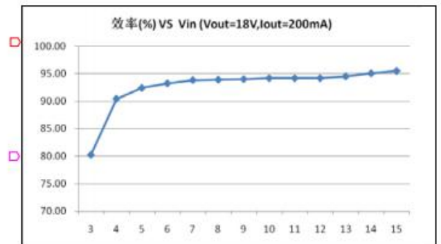
Efficiency VS Vin
