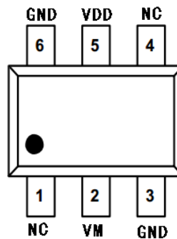
SOT23-6 TopView
