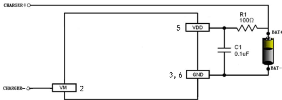
Fig 6 XB5306A in a Typical Battery Protection Circuit
